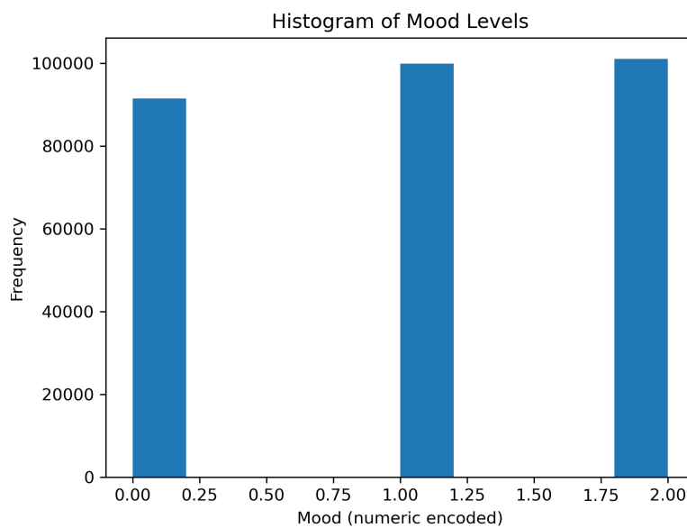
Figure 15: Mood Histogram.
