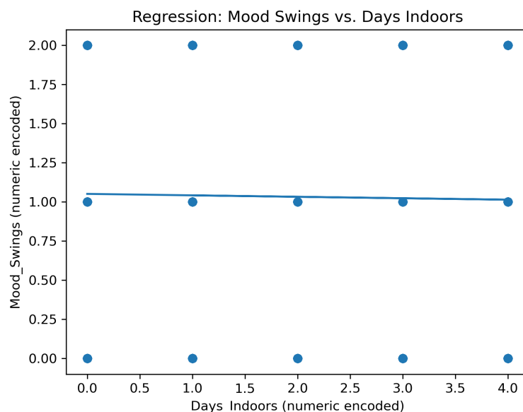
Figure 13: Regression Model.
