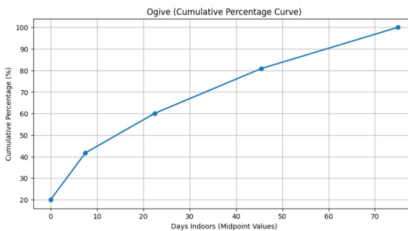
Figure 2: ogive charts.
